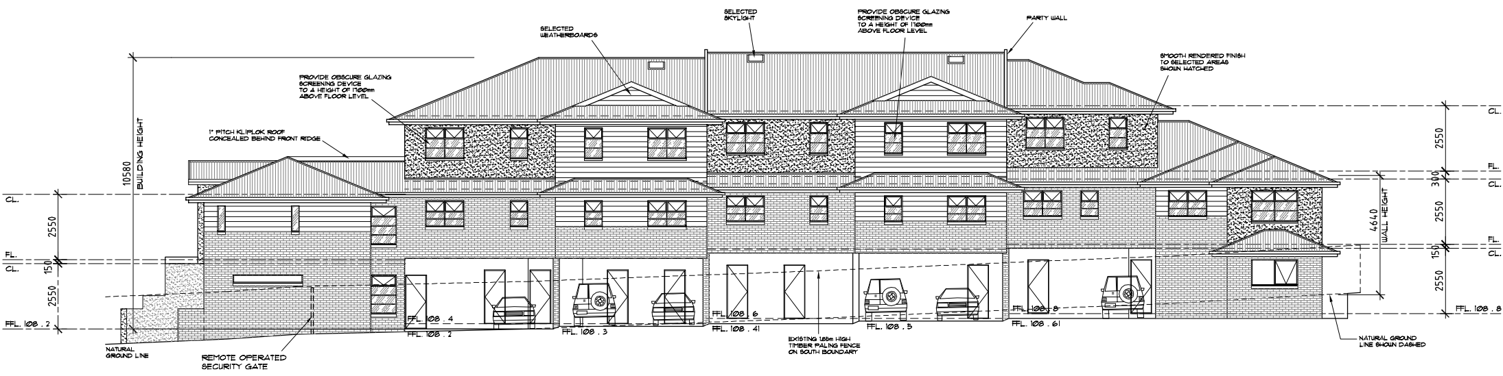
SOUTH SIDE ELEVATION 1:100
