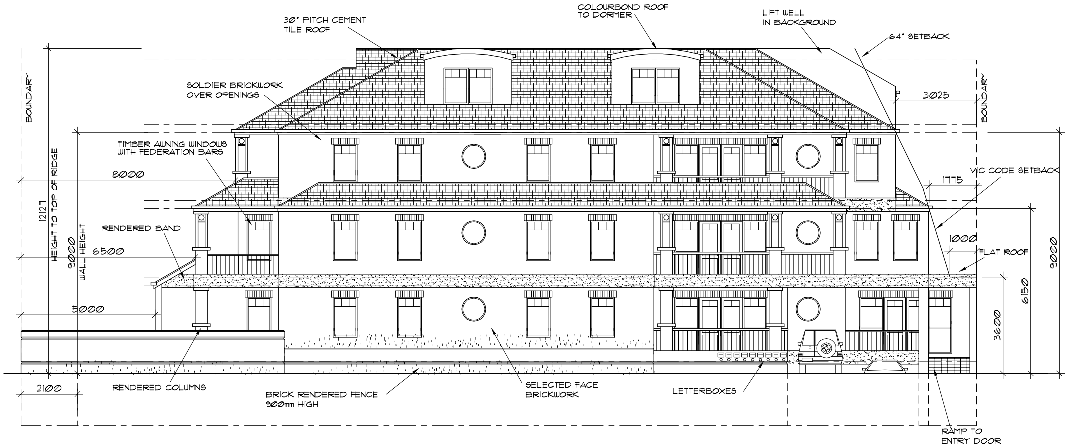
SOUTH ELEVATION 1:100
