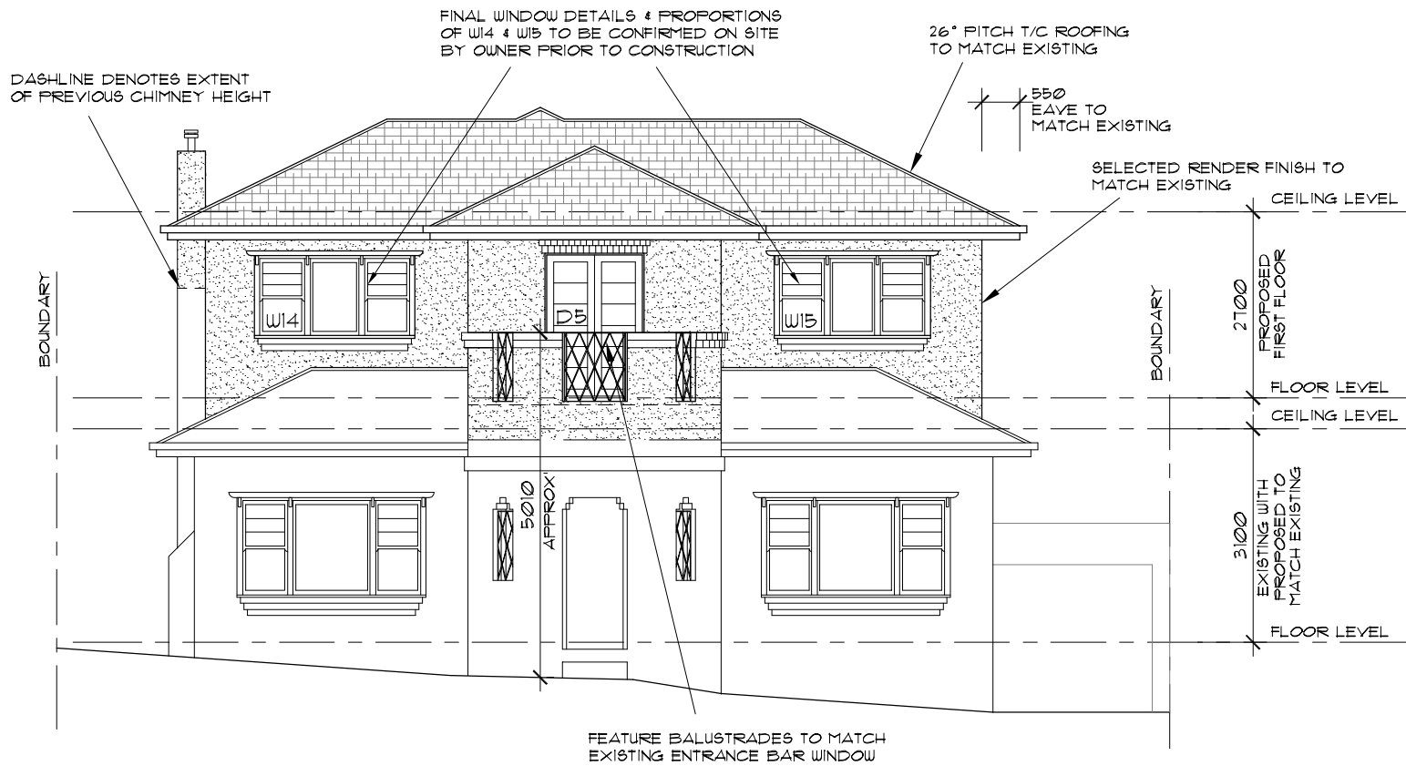
NORTH FRONT ELEVATION "1" 1 : 100
