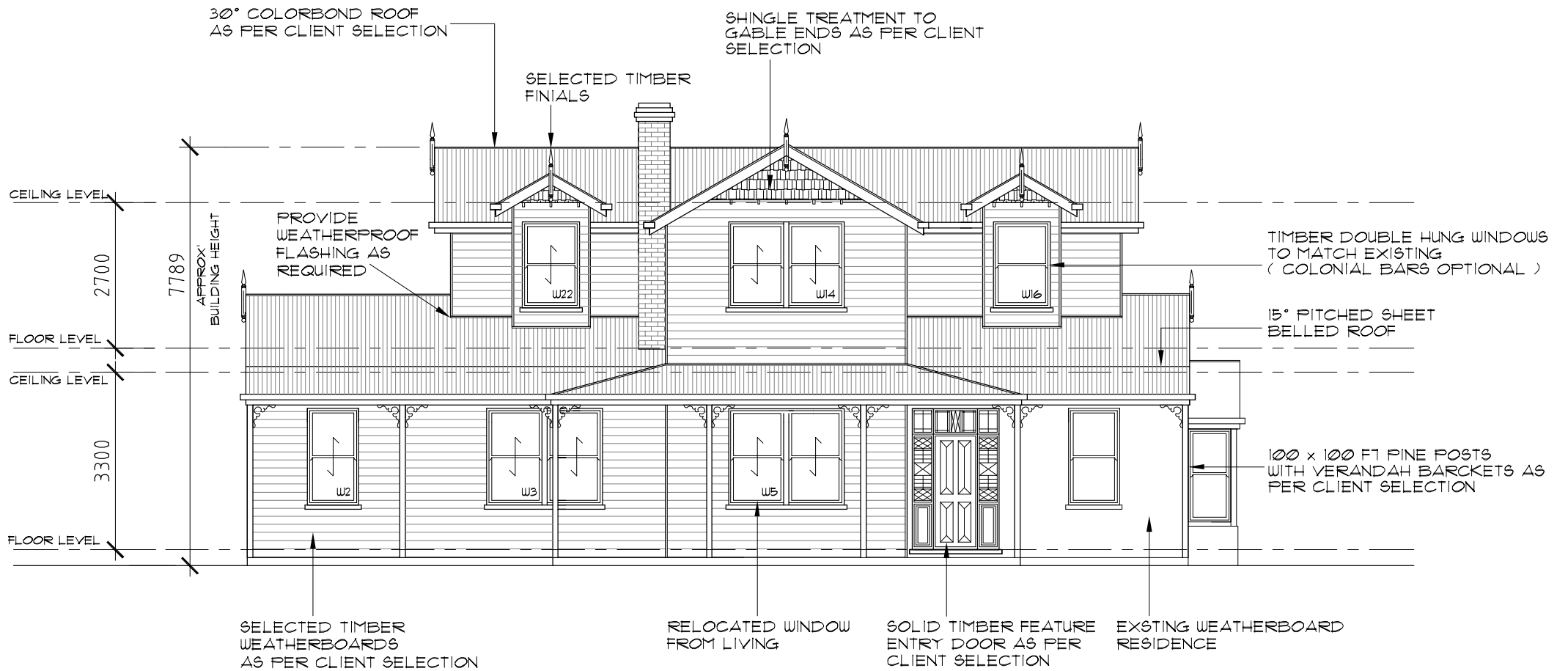
SOUTH FRONT ELEVATION " 1 " 1 : 100
