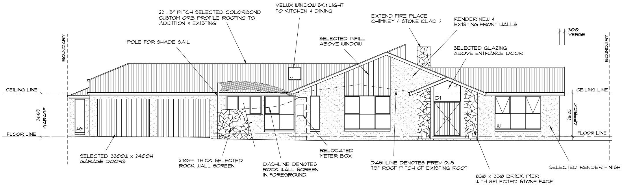
NORTH FRONT ELEVATION " 1 " 1 : 100
