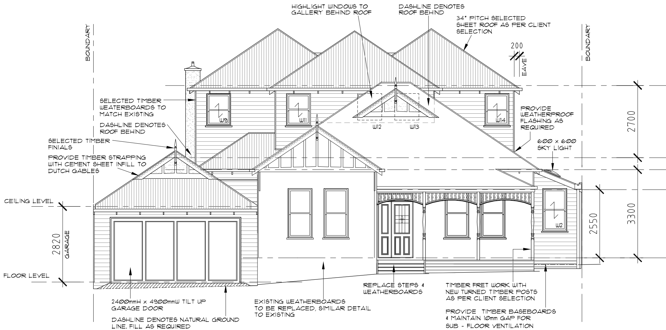
PROPOSED FRONT WEST ELEVATION " 1 " 1 : 100
