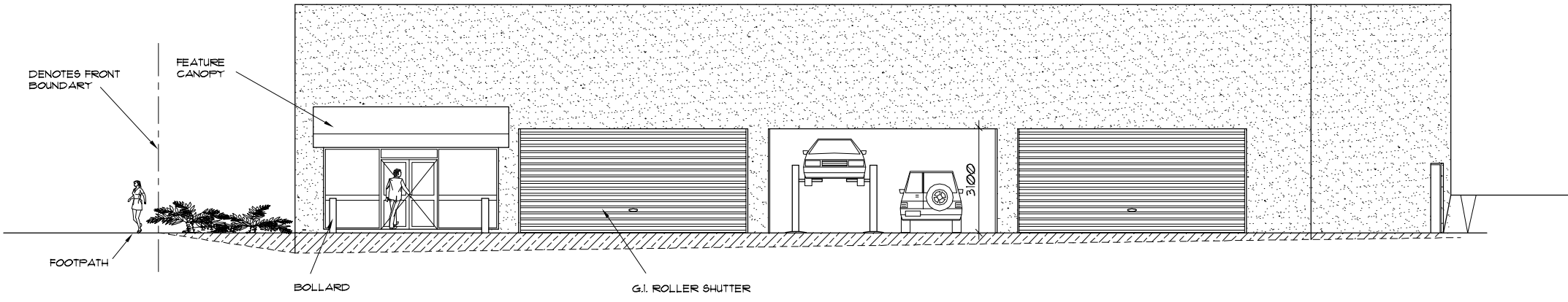
WEST SIDE ELEVATION 1:100
