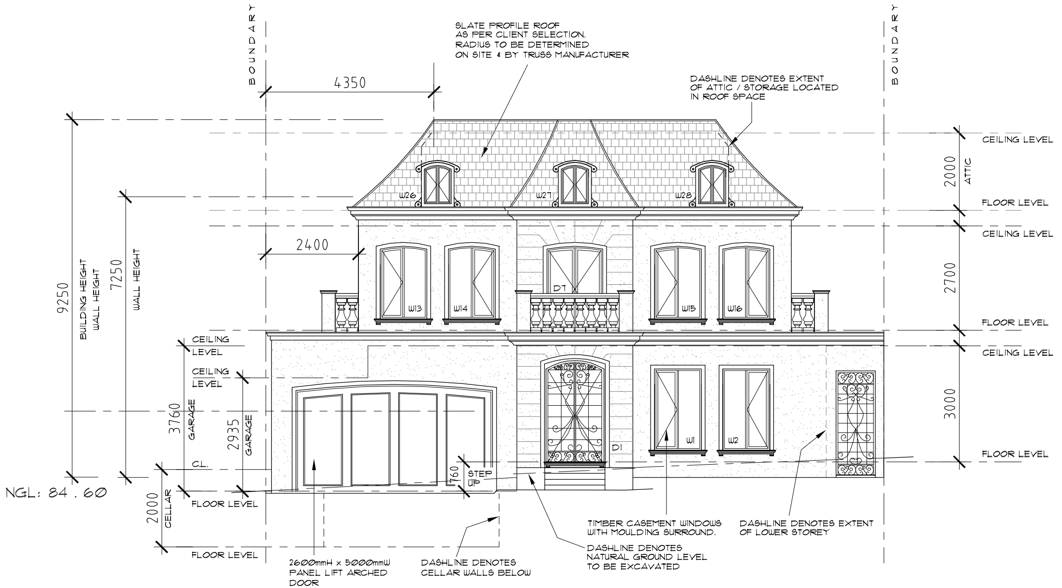
WEST FRONT ELEVATION " 1 " 1 : 100
