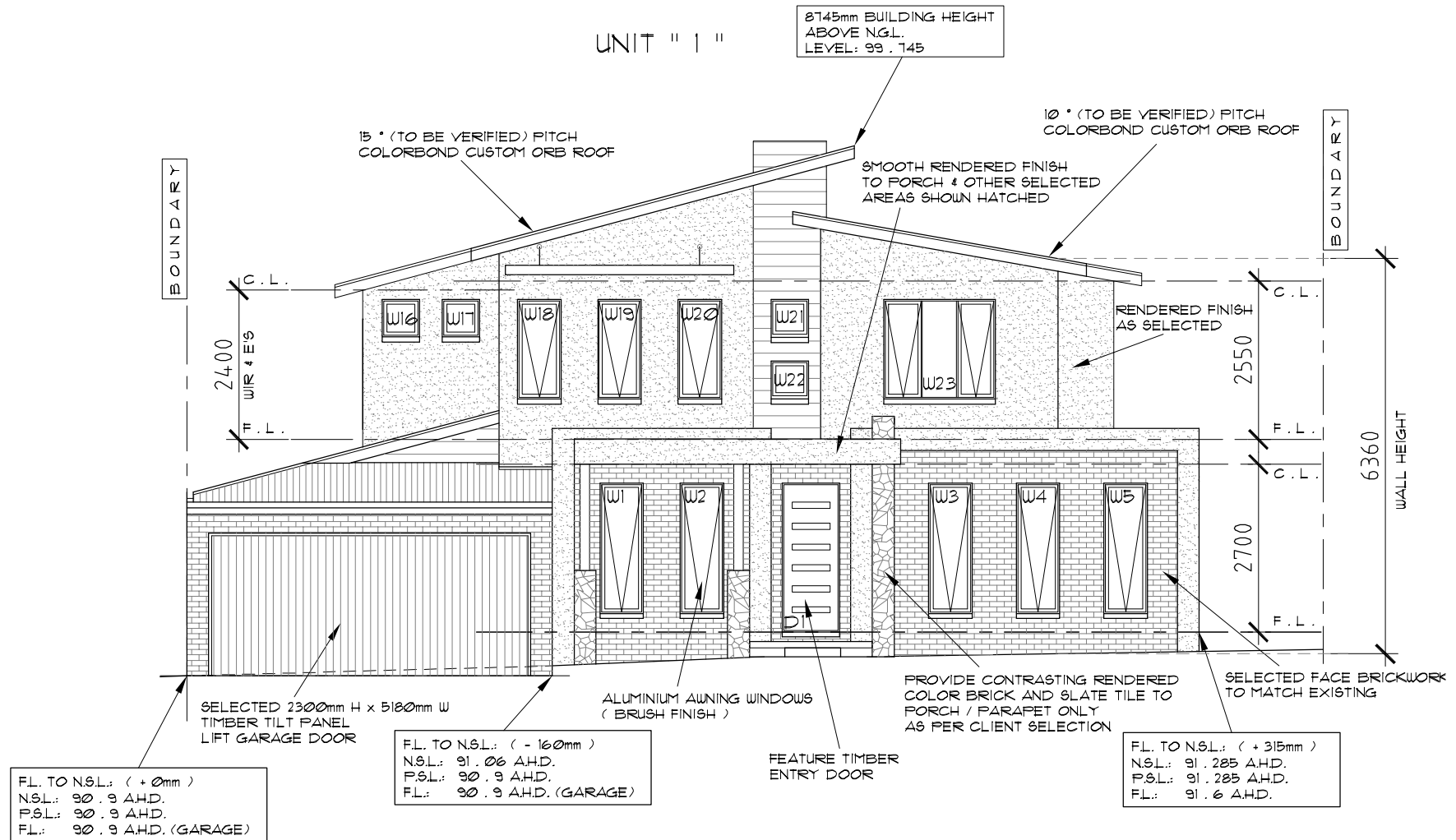
PROPOSED WEST FRONT ELEVATION 1 : 100 ( FACING SHEEHANS ROAD )
