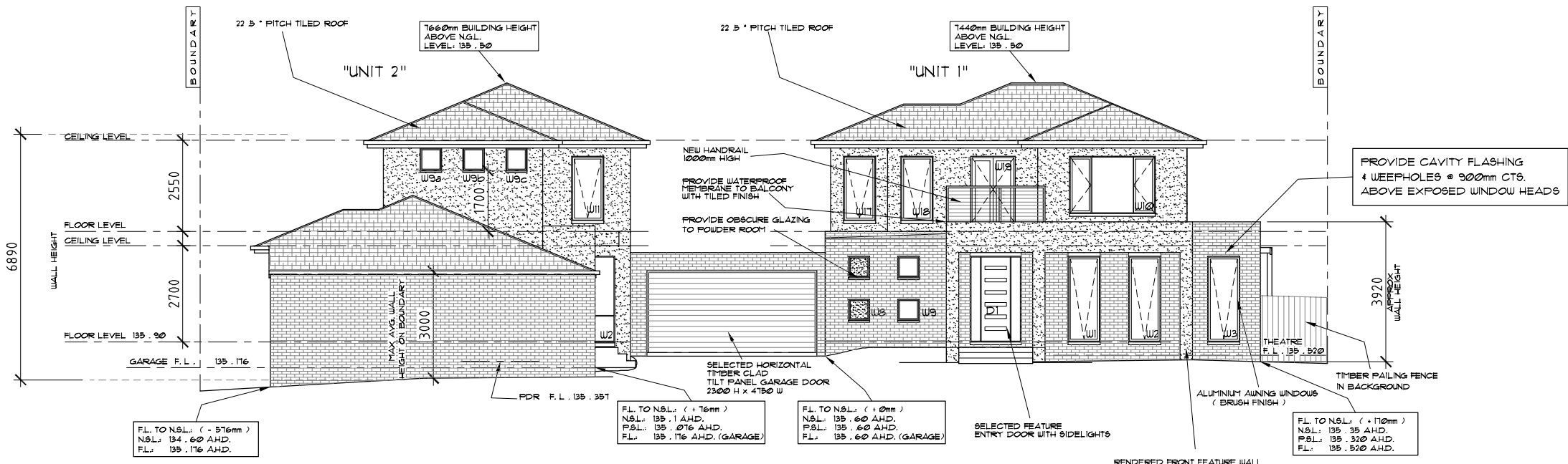
PROPOSED EAST FRONT ELEVATION 1:100
