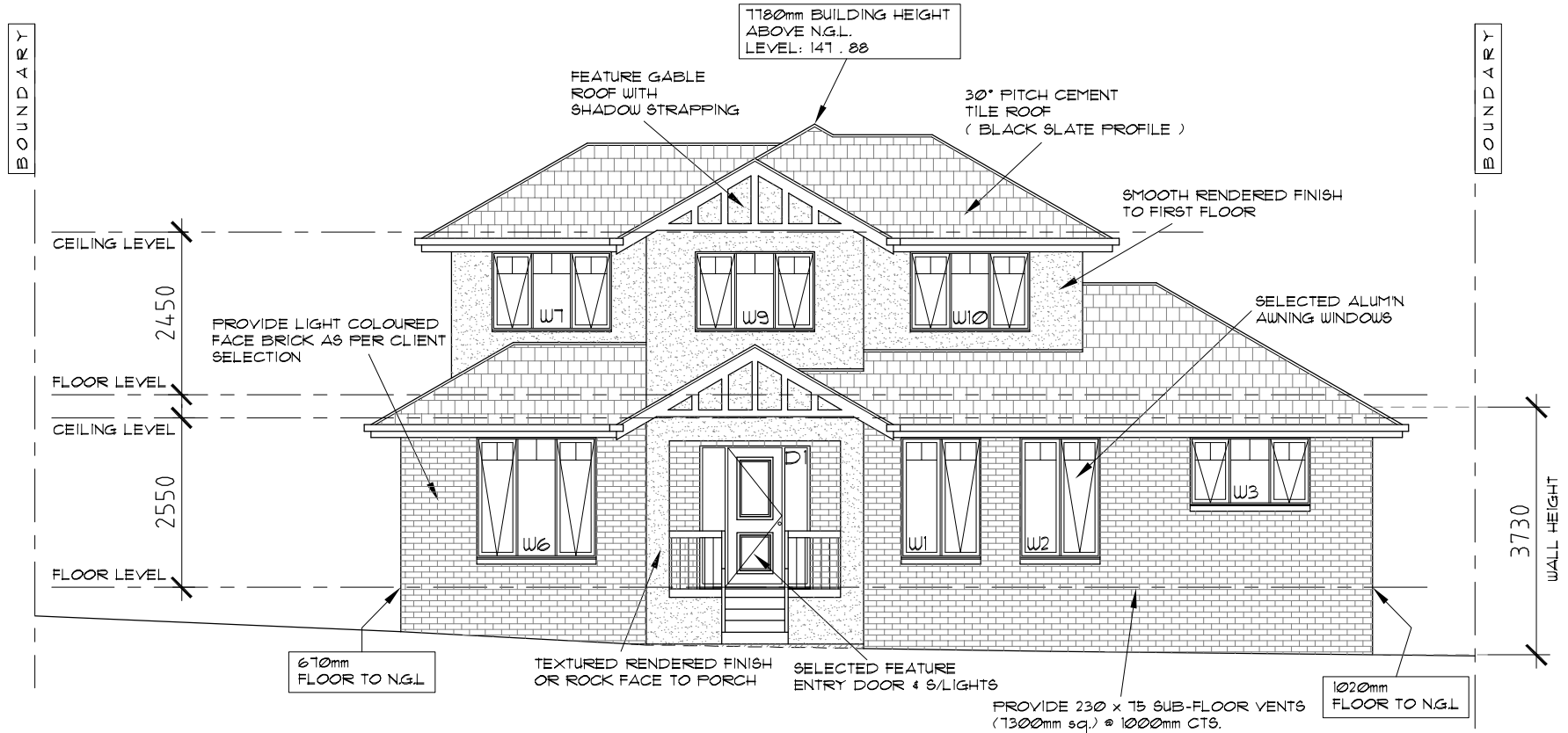
EAST FRONT ELEVATION 1 : 100 UNIT " 1 " ( FACING PERCY STREET )
