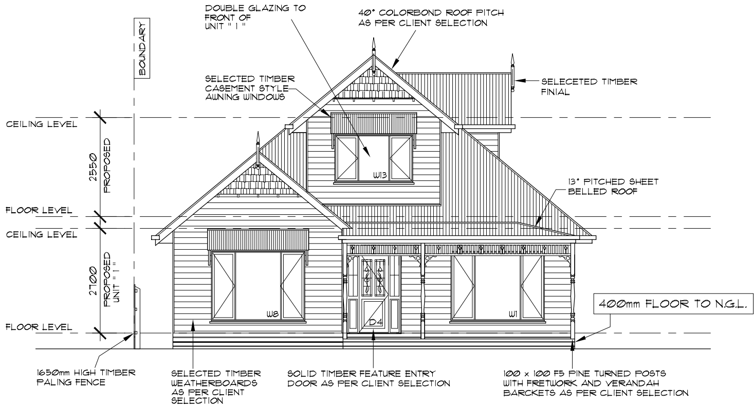
NORTH FRONT ELEVATION " 1 " 1 : 100 UNIT " 1 "
